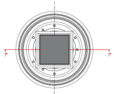
VERTICAL DRY White Glass Varijanta rešetke
